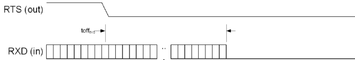
Figure 10-2: HCI UART receive flow control timing
