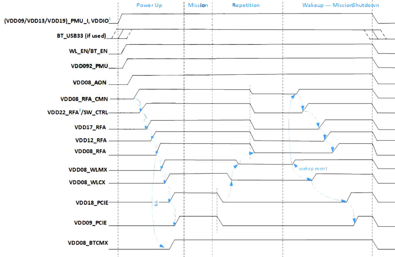
Figure 9-1: Module power sequences requirement
