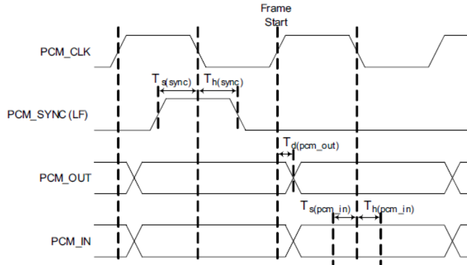
Figure 10-4: PCM interface timing diagram (master)
