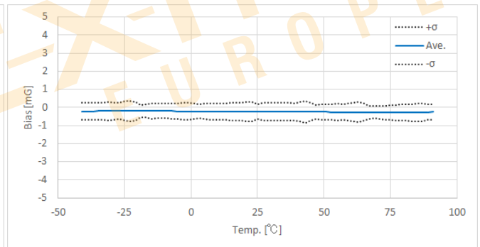
Figure 3.5 Accelerometer Bias vs. Temperature Characteristic (M-G370PDG0)
