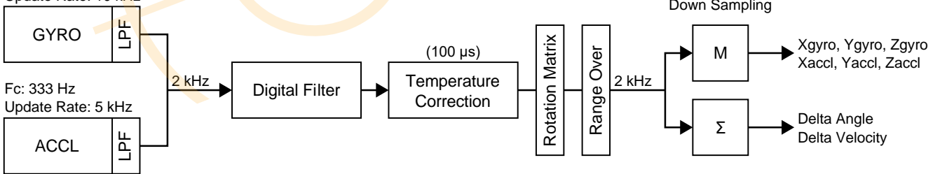
Figure 4.4 Functional Block Diagram
