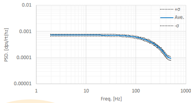
Figure 3.9 Gyro Noise Frequency Characteristic (M-G370PDT0)
