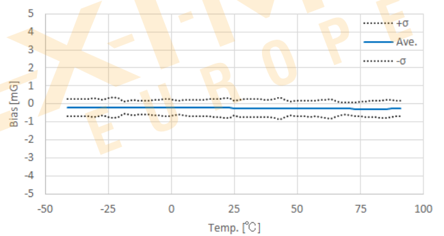
Figure 3.11 Accelerometer Bias vs. Temperature Characteristic (M-G370PDT0)
