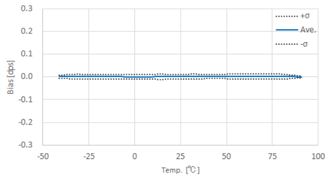
Figure 3.8 Gyro Bias vs. Temperature Characteristic (M-G370PDT0)
