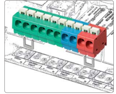
Customization which cannot be modified after soldering Bridges for short circuit to be inserted in the terminal block before soldering.
