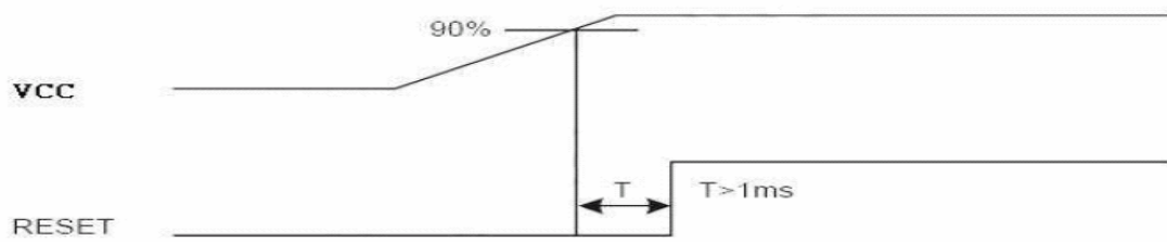
Reset timing
