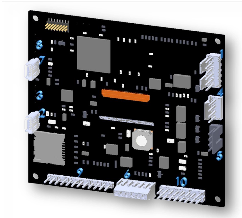
Figure 8: GTT35A Header Locations
