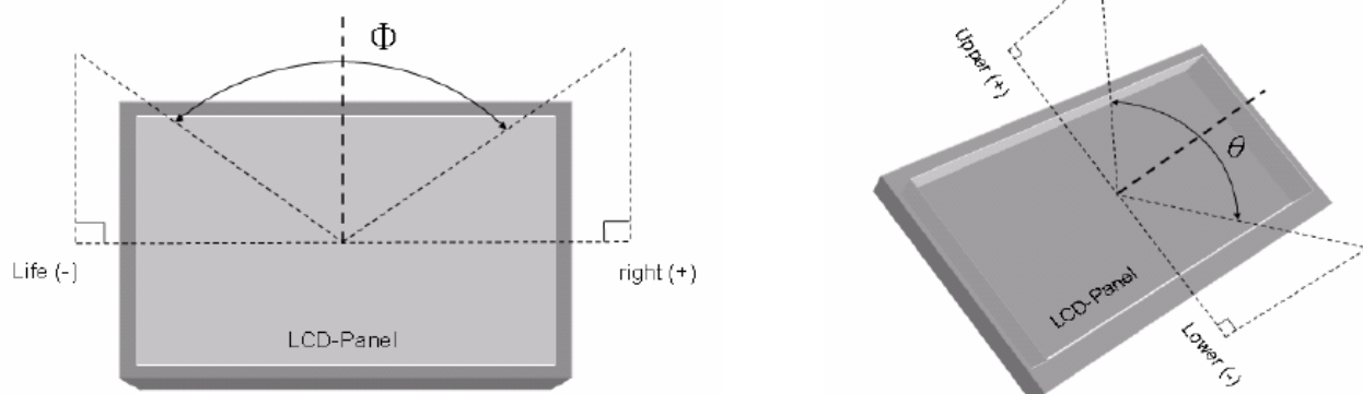
Fig9-2 Definition of Viewing Angle
