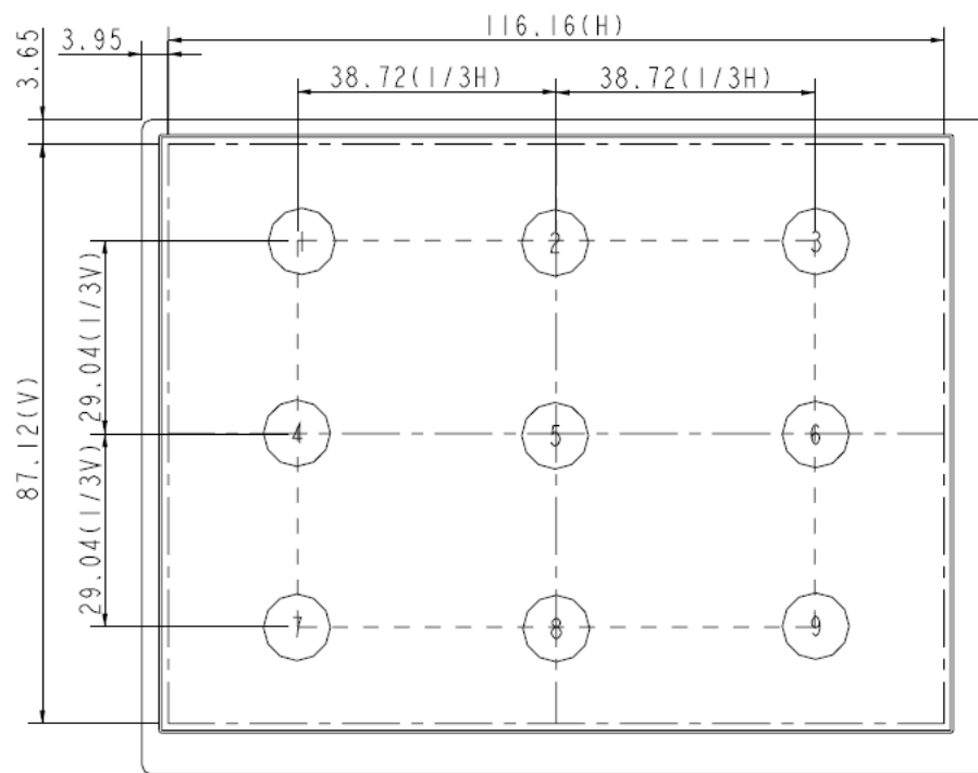
Fig9-1 Measuring point
