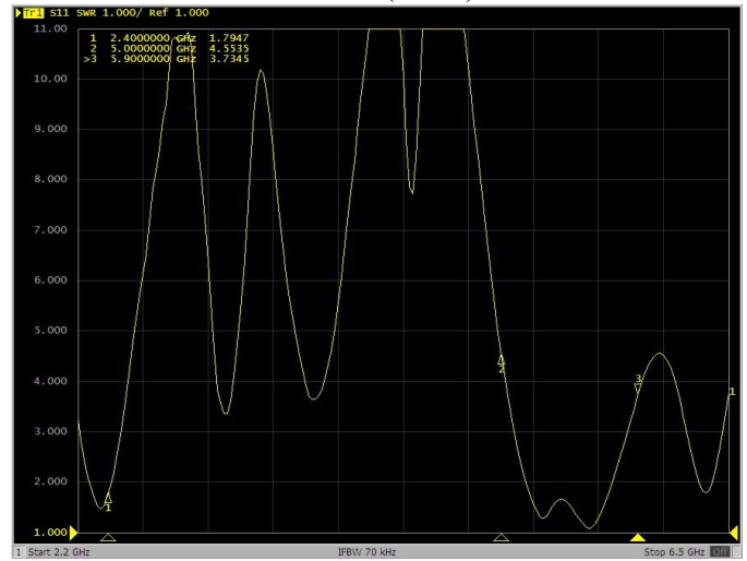
VSWR (WiFi)
