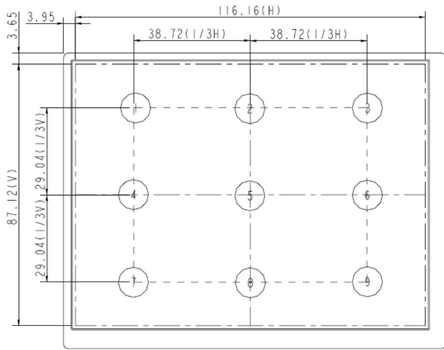
Fig9-1 Measuring point
