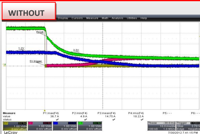
Figure 1: Sudden power outage WITHOUT iCell
