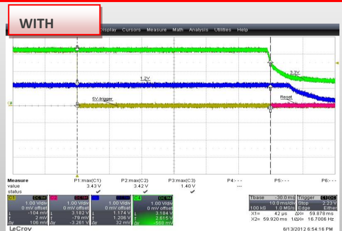
Figure 2: Sudden power outage WITH iCell Technology
