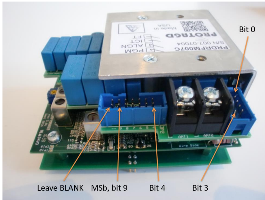
Figure 5.3 Jumper for Antenna Tuning
