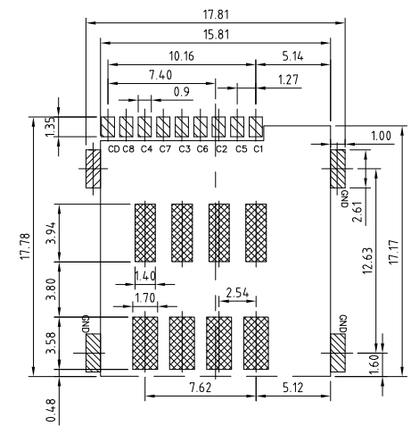
BOARD PAD NO WIRING AREA (TOLERANCES: ±0.05) RECOMMENDED PCB LAYOUT (8 PINS)
