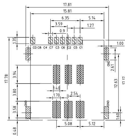
BOARD PAD NO WIRING AREA (TOLERANCES: ±0.05) RECOMMENDED PCB LAYOUT (6 PINS)
