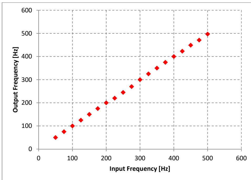
Fig. 8: Output frequency of acceleration vs. input voltage signal frequency for 10 pulses. Input voltage has a single pulse half wave sinus signal form of amplitude 0 to 60 V and varying frequency from 50 to 500 Hz. The frequency of output acceleration is calculated.
