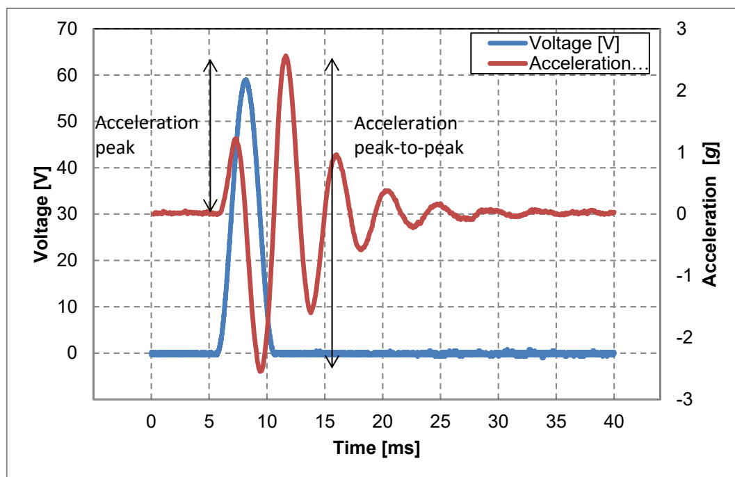
Fig. 5: Typical acceleration g as a function of input voltage with 100 g load. Input voltage with a half wave sinus signal form of amplitude 0 to 60 V and pulse length 5 ms which is equivalent to 200 Hz.
