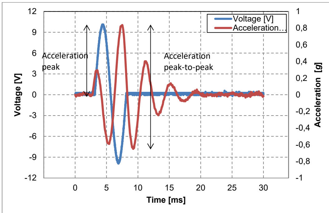
Fig. 6: Typical acceleration g as a function of input voltage with 100 g load. Input voltage with a sinus signal form of amplitude -10 to 10 V and pulse length 5 ms which is equivalent to 200 Hz.
