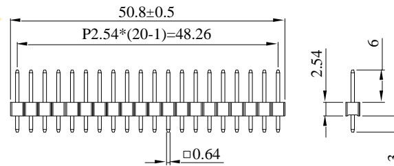
Pin Detail SCALE 1/1
