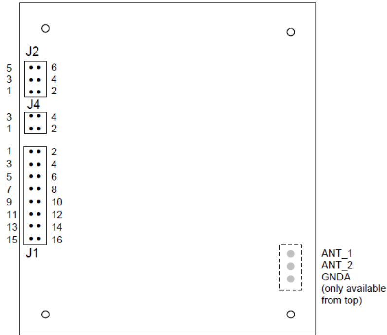
Figure 4.4 PRDRFM008B Bottom View
