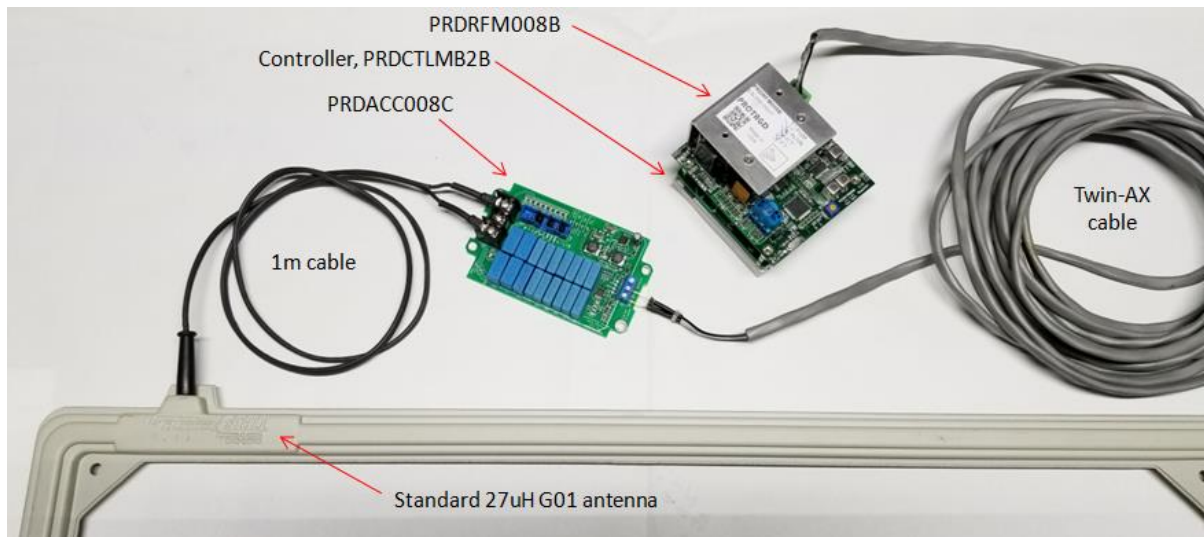
Figure 5.1 Connections
