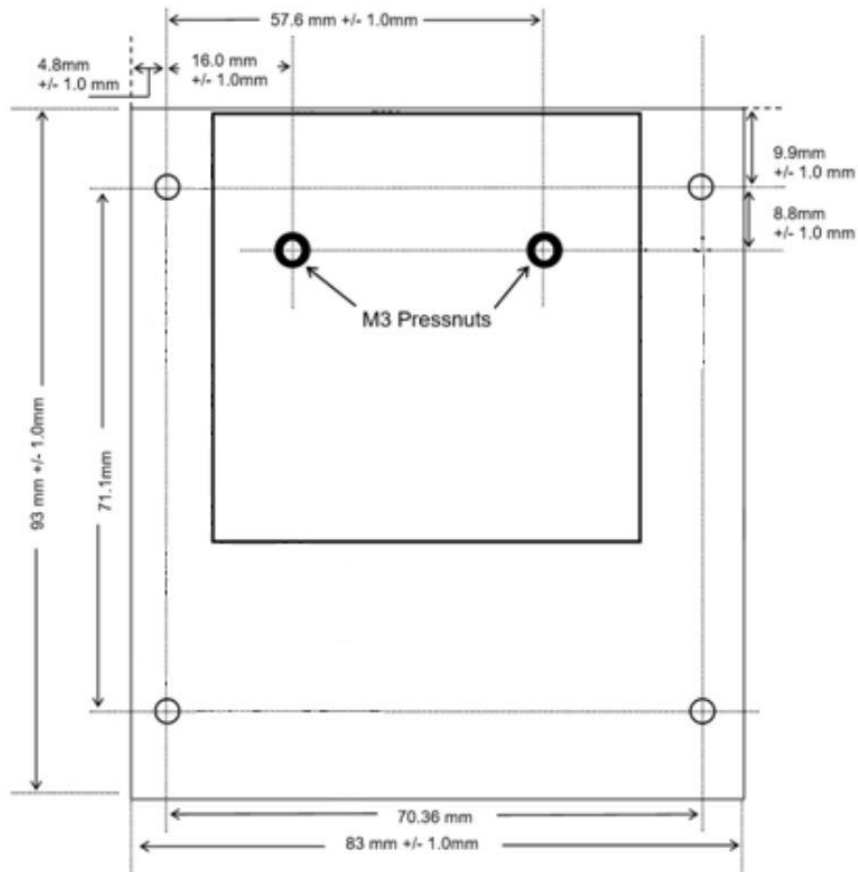
Figure 6.1 Mechanical Dimensions PRDRFM008B
