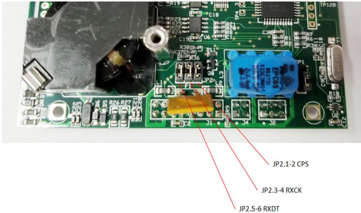
Figure 5.6 Other Jumpers
