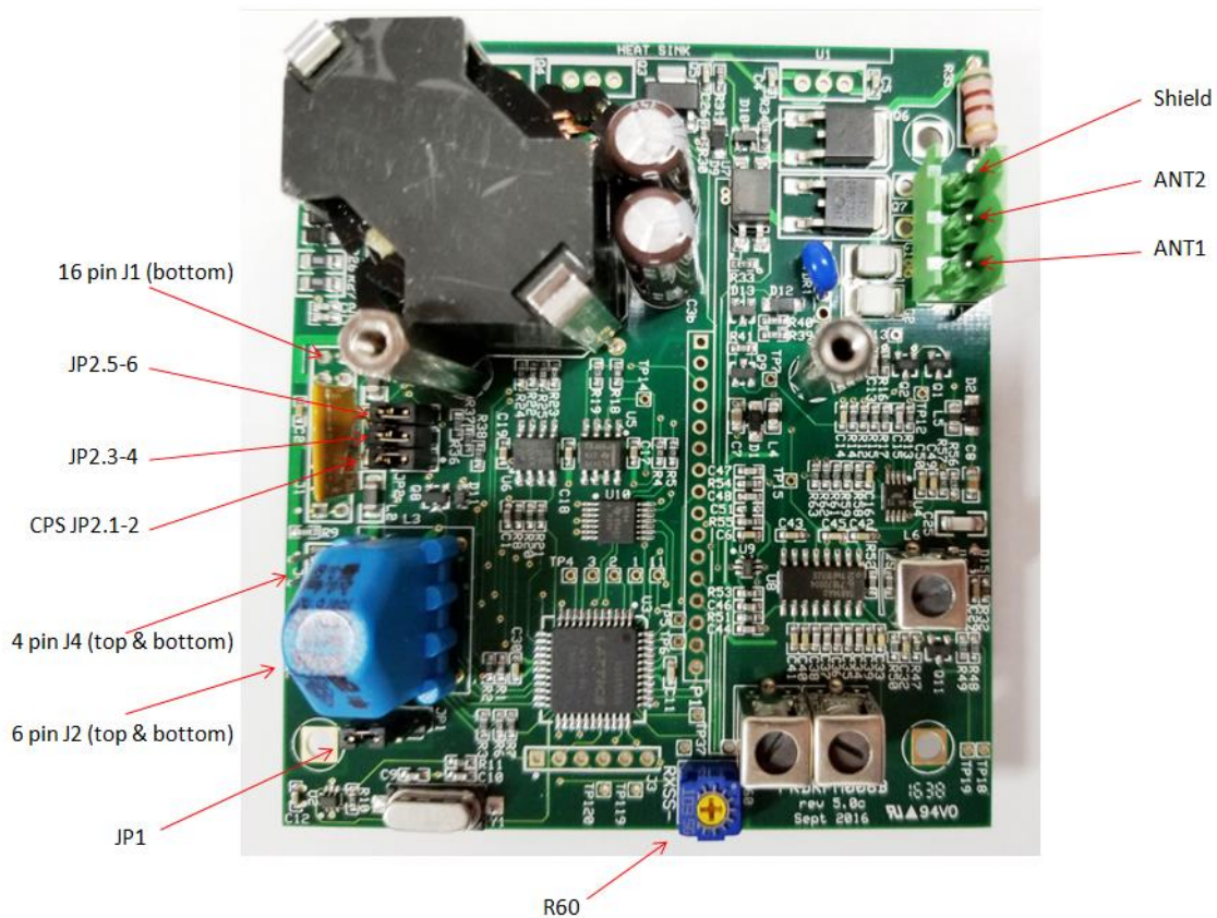
Figure 4.2 PRDRFM008B Top View
