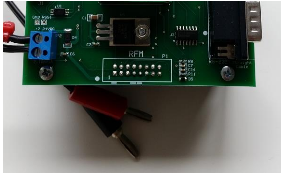
Figure 5.3 Power Supply Connected to PRDBIF1 Controller
