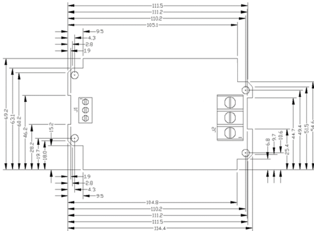
Figure 6.2 Mechanical Dimensions PRDACC008C
