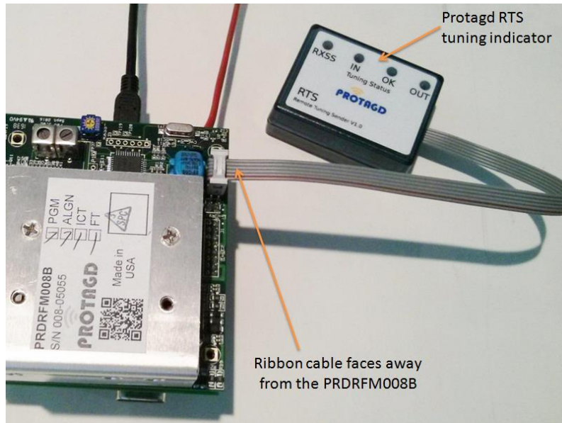
Figure 5.2 RTS Connection
