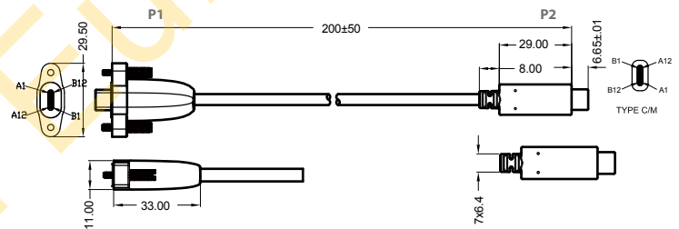
Waterproof USB-C to Standard USB-C Cable P/N : 9480240240K2
