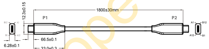
Standard USB-C Cable P/N : 9480240240K7
