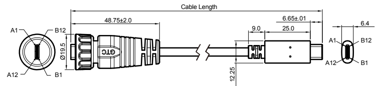
Waterproof USB-C to Standard USB-C Cable P/N : 9480240240K2
