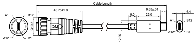
Waterproof USB-C to Standard USB-C Cable P/V : 9480240240K2
