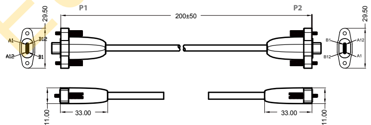
Waterproof USB-C to Lockable USB-C Cable P/N : 9480240240K8
