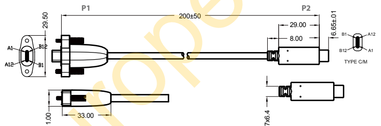
Lockable USB-C to Standard USB-C Cable P/N : 9480240240K5
