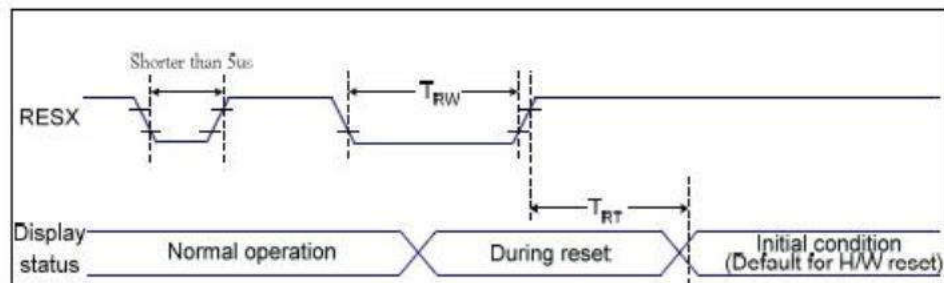
Figure 7 Reset Timing
