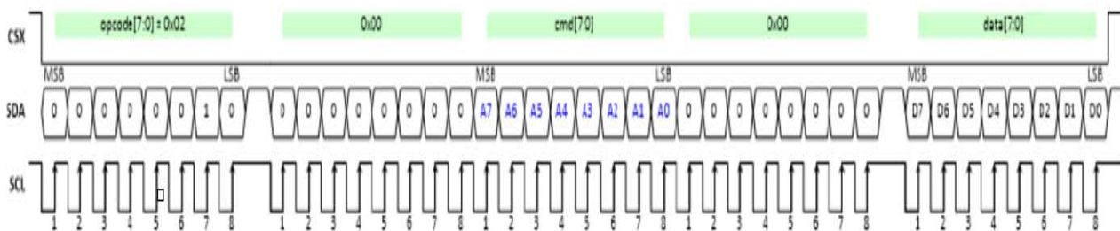
QSPI write command and write data (1 data lane)
