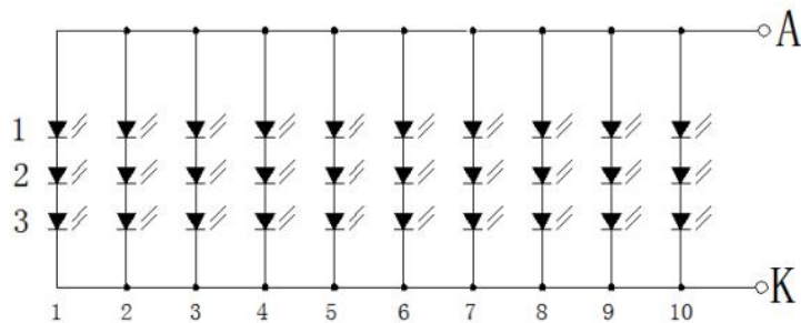
Fig. 3-1 LED test circuit diagram
