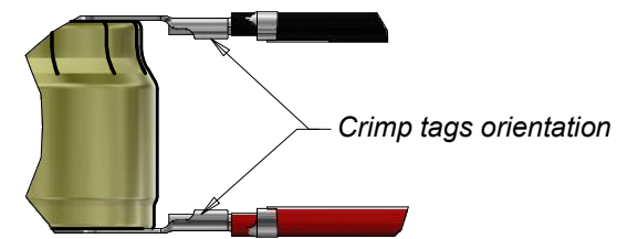
View A Scale 5 : 1
