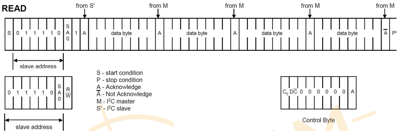
Figure 7 I 2 C Protocol
