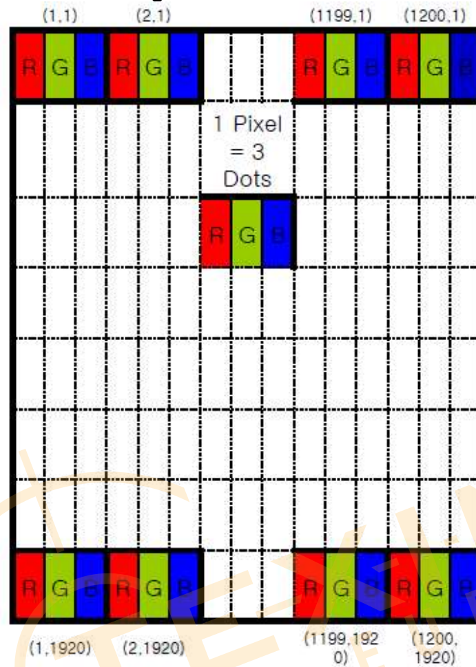
Figure 1. Pixel Format
