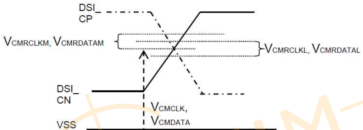
Figure 2: Differential voltage range and Command mode voltage
