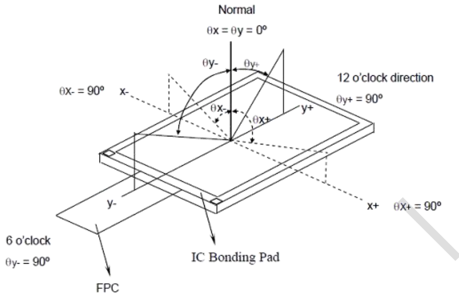
Note 8: Optical characteristic measurement setup.
