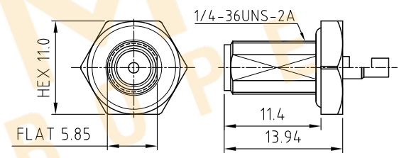
SMA JACK DETAIL DRAWING
