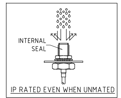
SMA JACK DETAIL DRAWING
