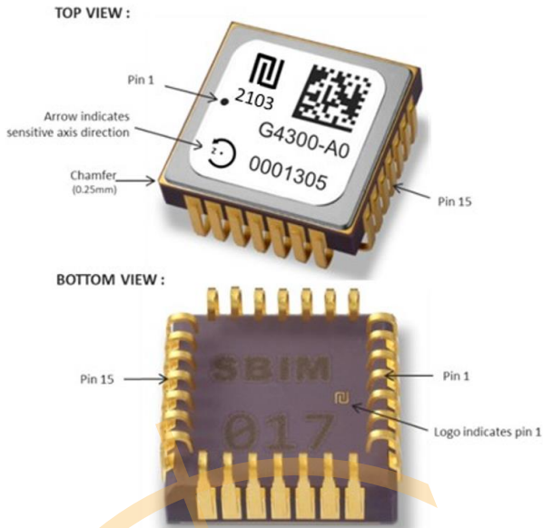
Figure 12: How to locate Pin 1
