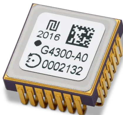
Figure 29: GYPRO4300 package
