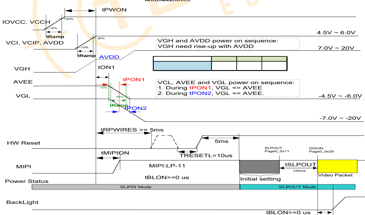
Figure 9.10: Power off sequence for differential power mode
