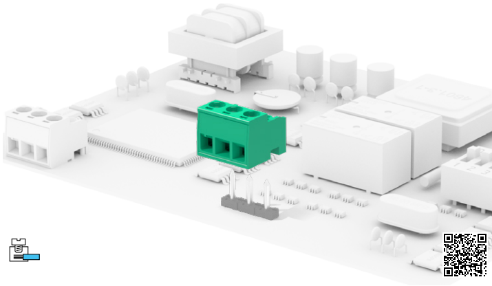
90°-270°, side stackable with snap features CSF_0S1 - 2 ÷ 25 poles, 5 mm / .197" pitch CSF_0S2 - 2 ÷ 13 poles, 10 mm / .394" pitch
