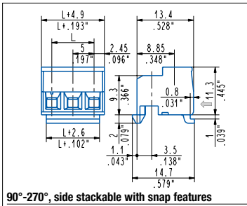
90°-270°, side stackable with snap features CSF_0S1 - 2 ÷ 25 poles, 5 mm / .197" pitch CSF_0S2 - 2 ÷ 13 poles, 10 mm / .394" pitch
