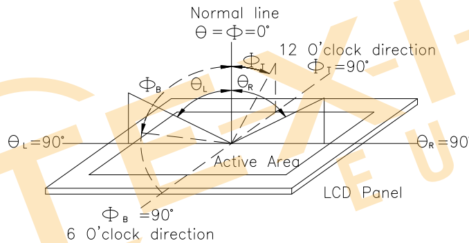
Fig. 6.1. Definition of viewing angle
