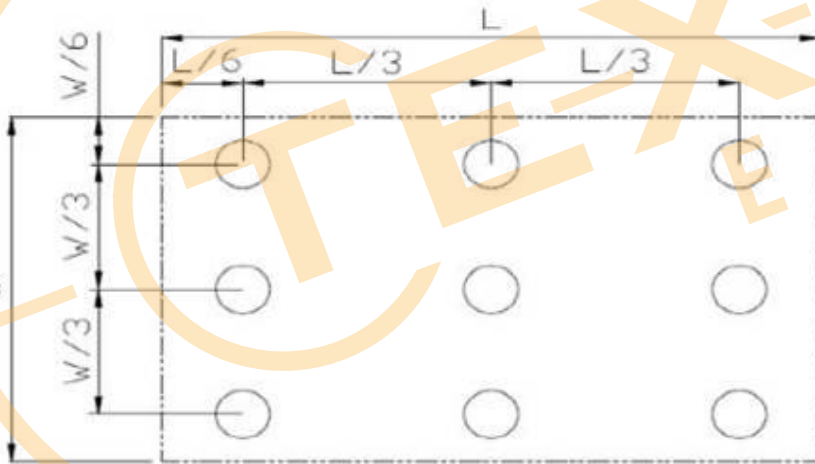
Fig 6.3. Definition of uniformity
