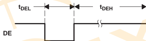
Figure 14. Minimum DE Low and Maximum DE High
