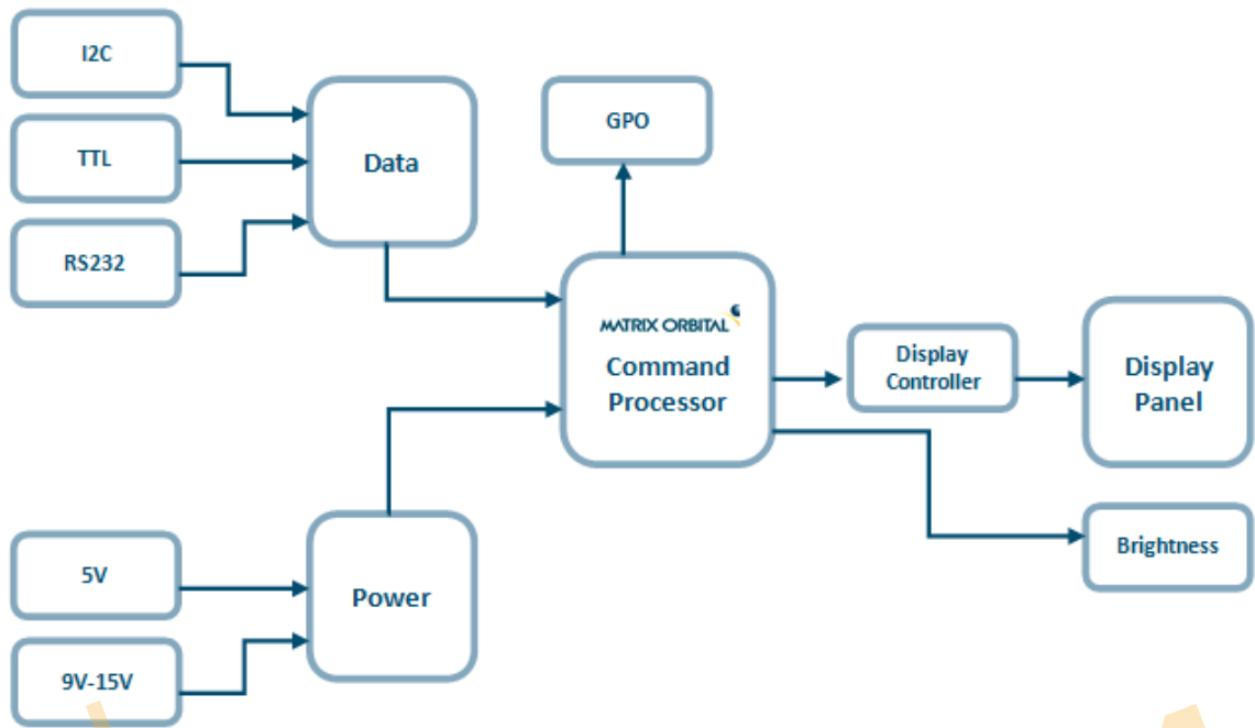
Figure 10: Functional Diagram
