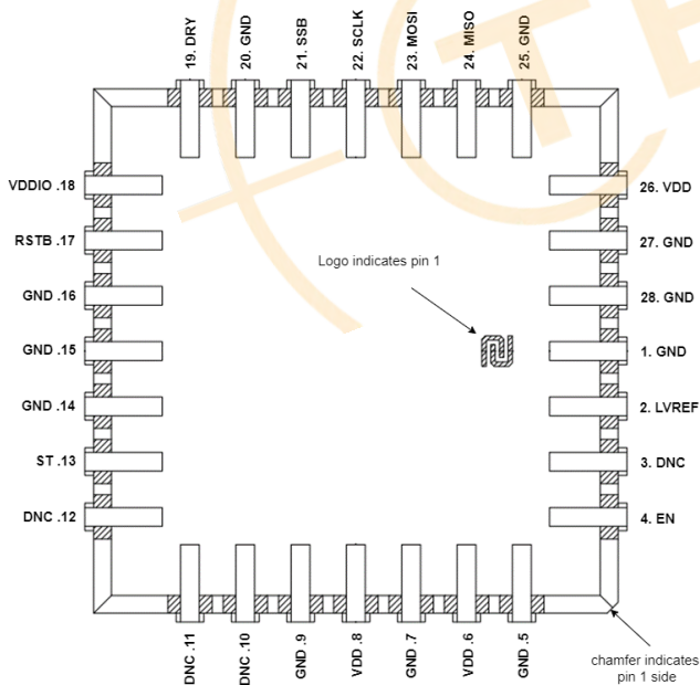
Figure 14: AXO305 Sensors Pinout (bottom view)
