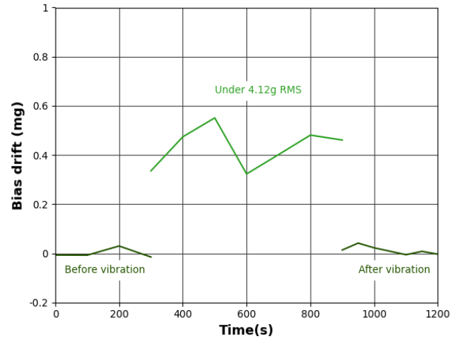
Figure 10: Bias drift under vibration
