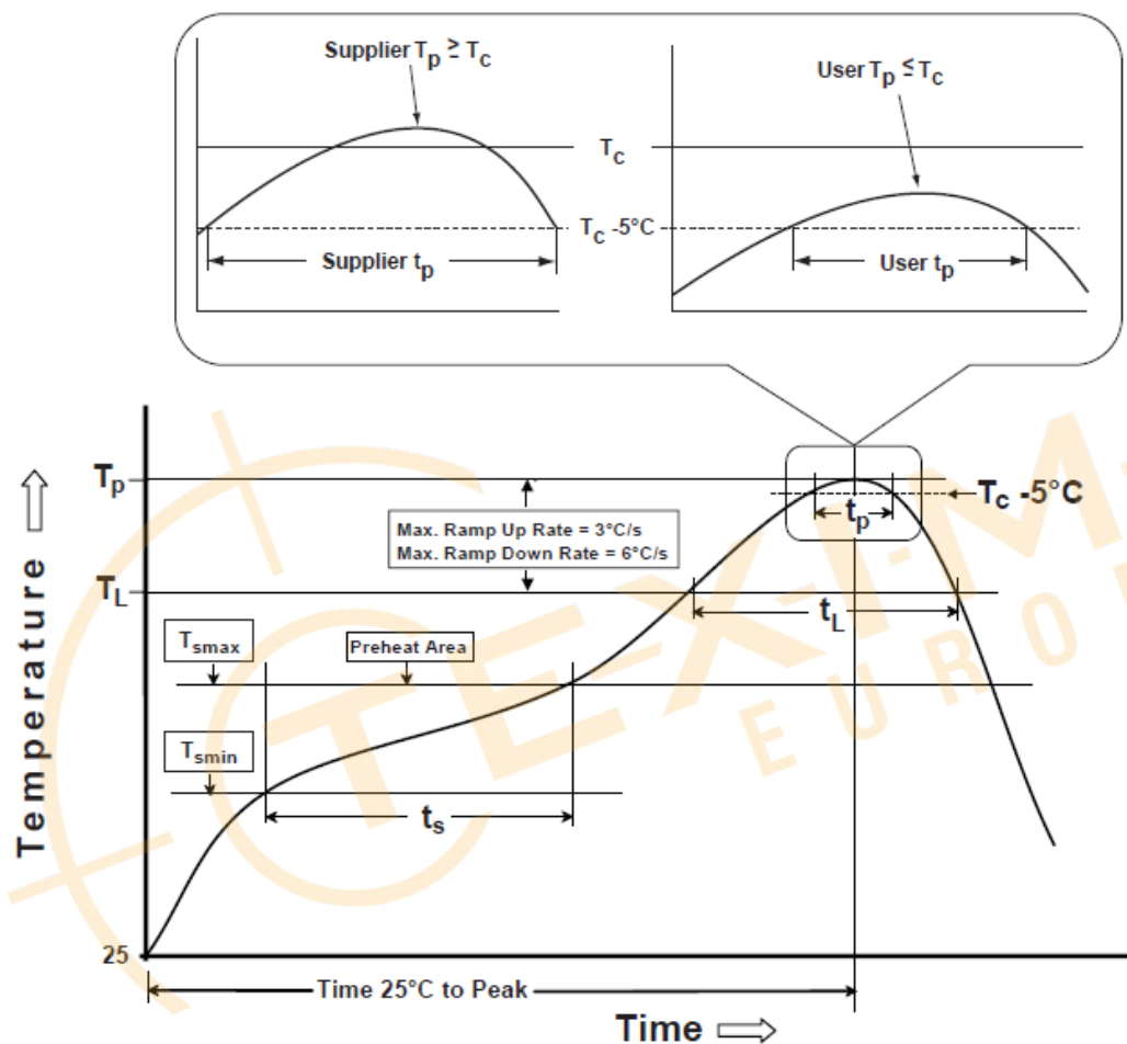
Figure 17: Recommended Reflow Profile, according to IPC/JEDEC J-STD-020D.1
