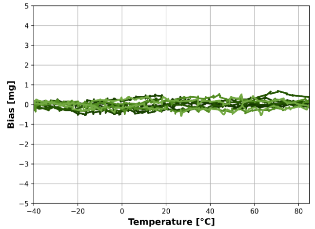
Figure 7 : Residual bias temperature error (5 samples)
