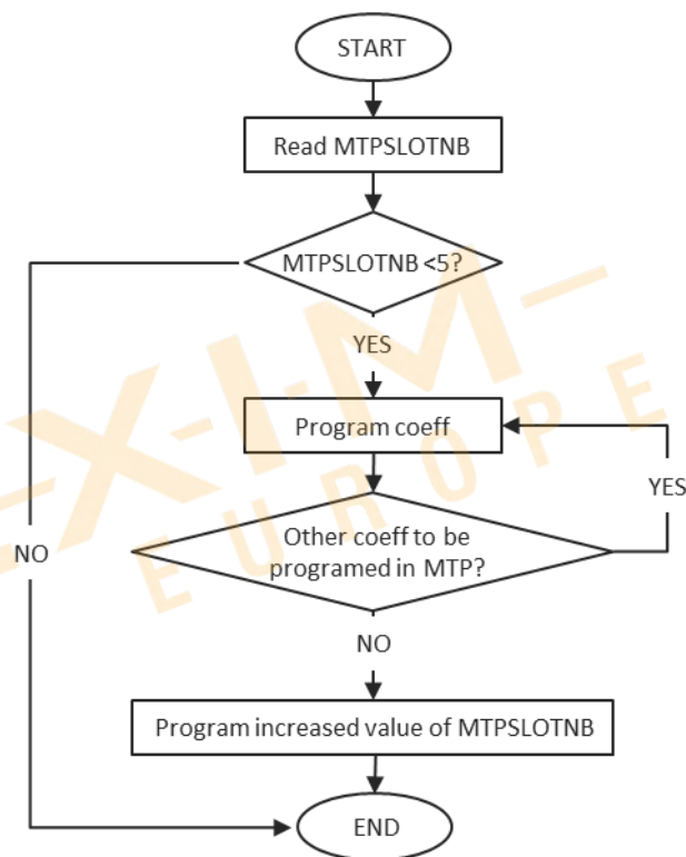
Figure 27: Procedure to program new calibration parameters
