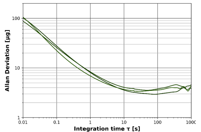
Figure 9: Allan variance (5 samples at 35°C)
