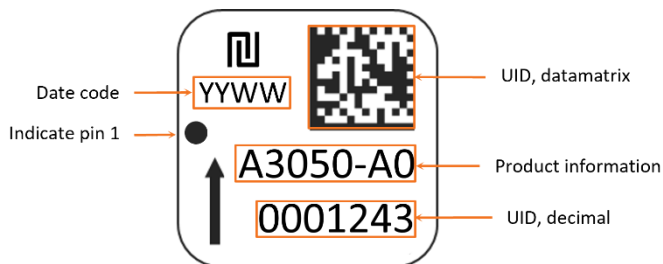
Figure 28: AXO305 label
