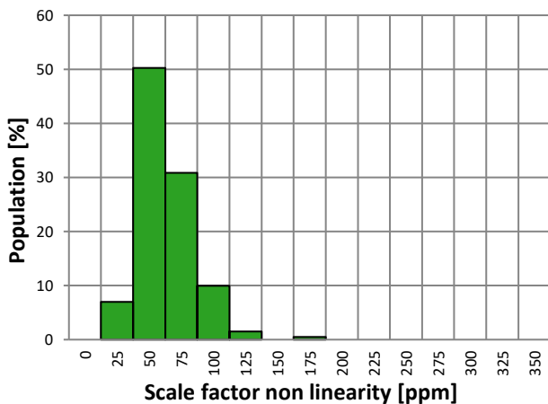
Figure 6: Scale Factor non linearity distribution (room temperature)
