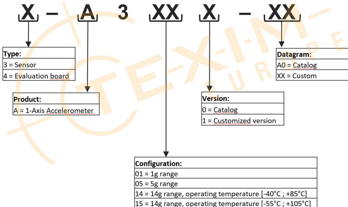
Figure 29: Ordering information
