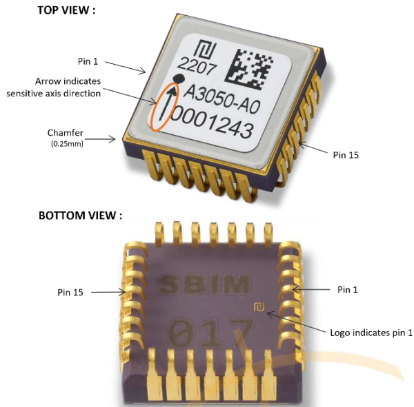
Figure 13: How to locate Pin 1 and Sensitive Axis
