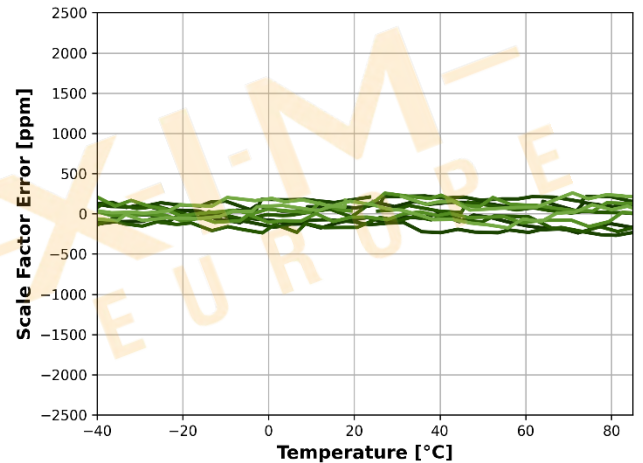
Figure 8: Residual scale factor error (5 samples)
