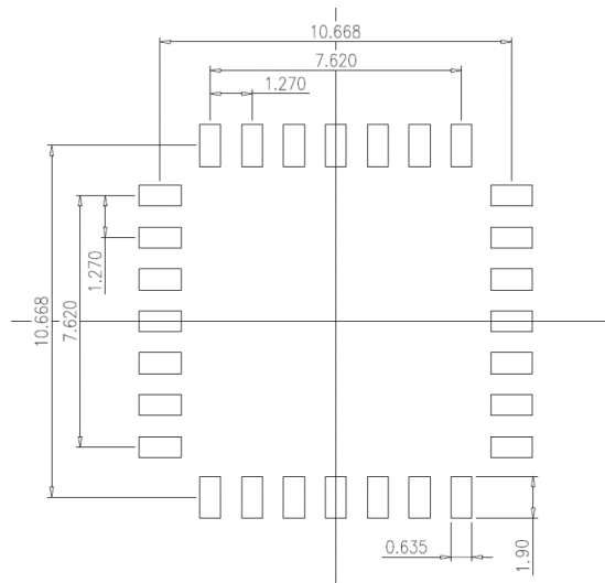
Figure 16: Recommended Pad Layout in mm (dimensions in mm)
