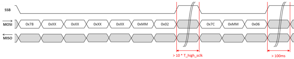
Figure 25: Sequence of instructions to WRITE data '0xXXXXXXXX' to address '0xMM' of the MTP
