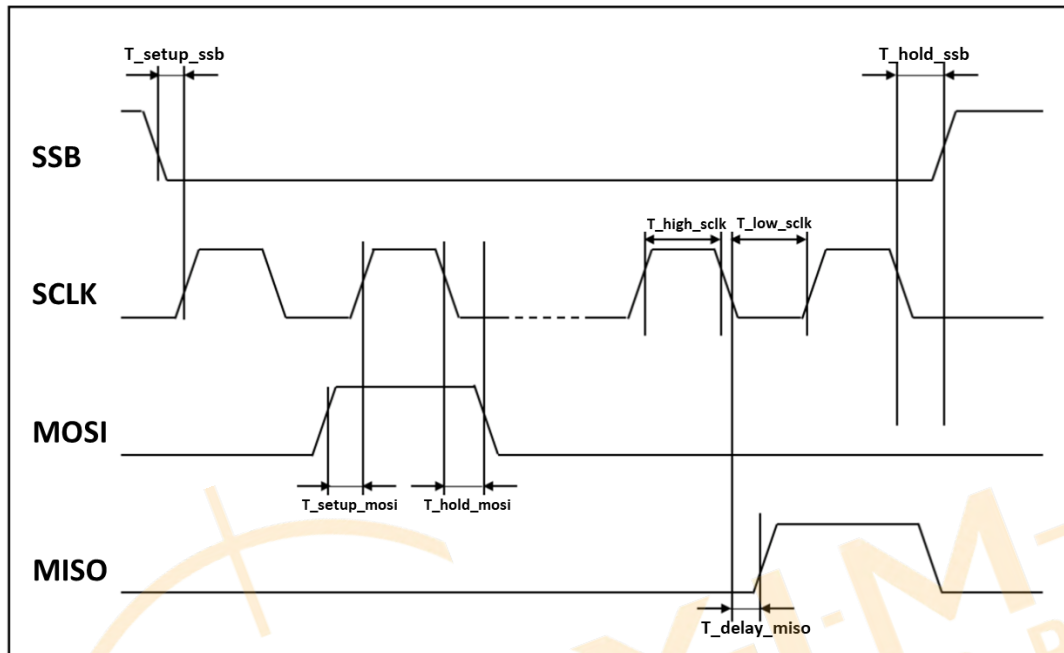
Figure 18: SPI timing diagram
