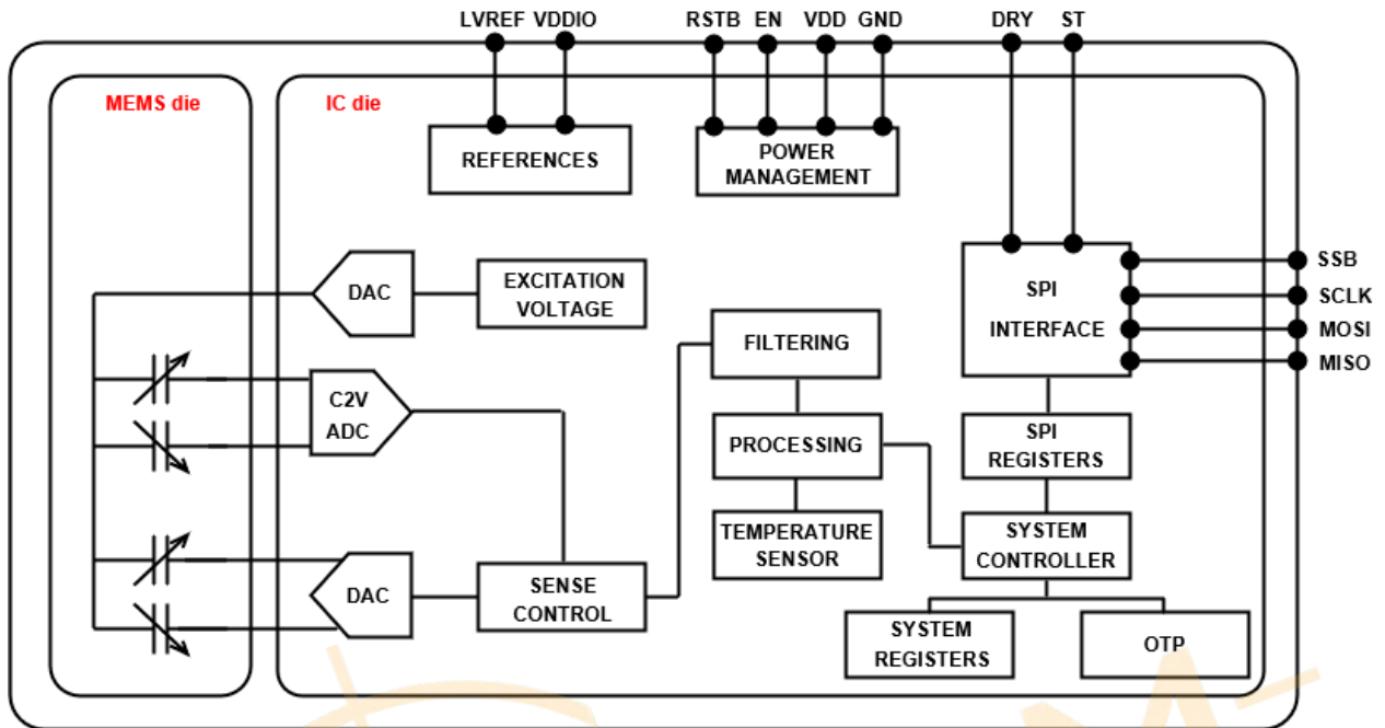
Figure 1 : Block Diagram
