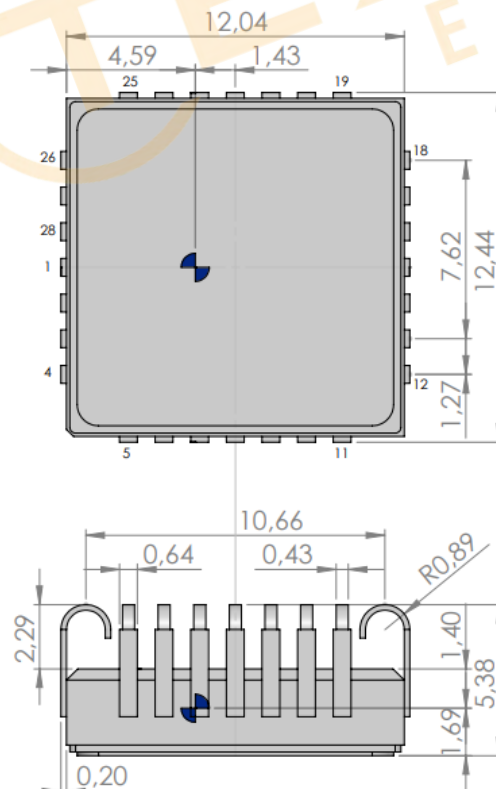
Figure 2 : Overall dimensions
